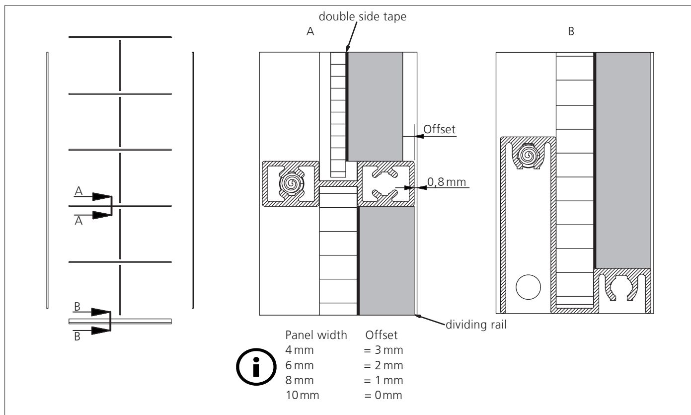
1_ continuous horizontal dividing rail with diverse panel widths (available as screwed version)
