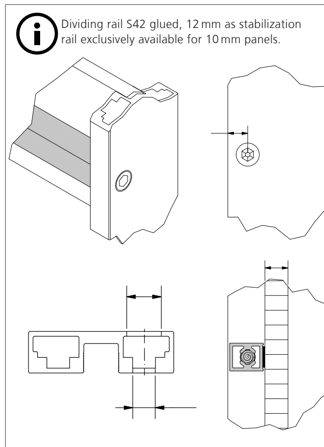
2_ Versaion as stabilization rail (screwed)
