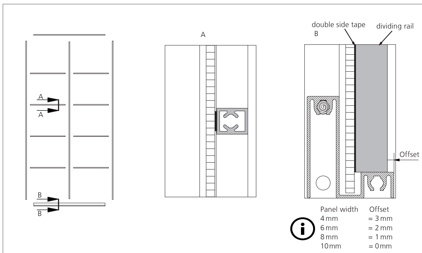
2_ continuous vertical dividing rail (all dividing rails only for gluing available)
